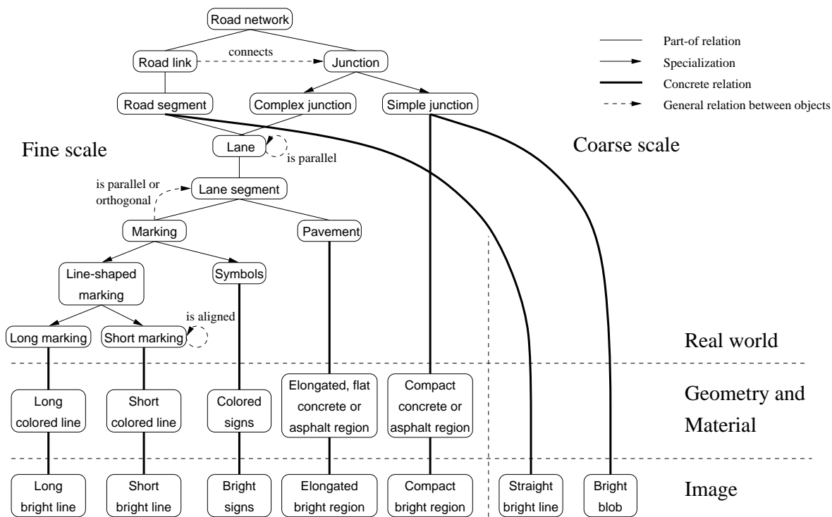
Figure 2: Road model
