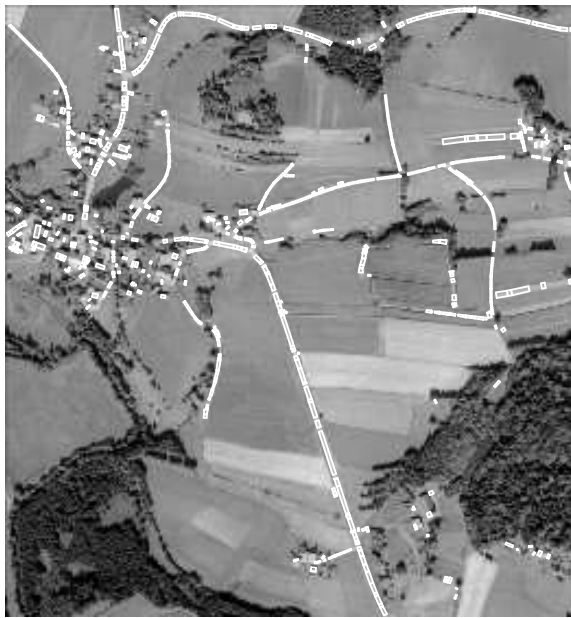
Figure 8: Road segments
