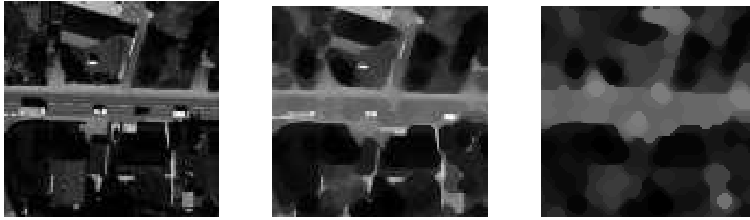
Figure 11: Car on road in morphological scale-space — Images (from left to right: original image, result of closing alone and of closing as well as opening - radius of disk = 1.5 m)
