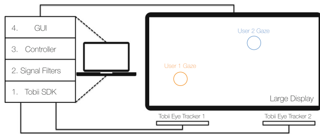
Fig. 2 The application receives gaze data from two eye tracking devices. Upon receiving the gaze data, the application first preprocesses the data and then informs the controller to update the positions of users' gaze visualisation on the user interface
