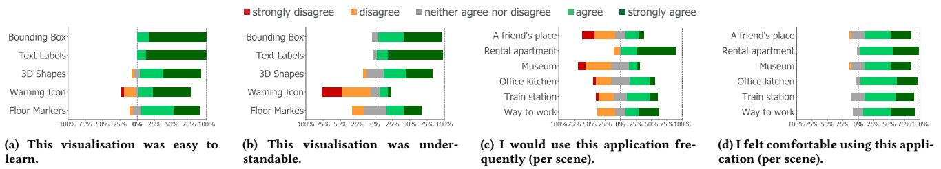
Figure 7: Study Part II (using PriView in an HMD in various scenes): Likert Ratings per visualisation for a) learnability and b) understandability; and per scene for c) frequent use and d) comfort.
