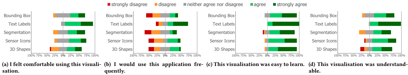
Figure 6: Study Part I (using PriView in a mobile application): Likert Ratings per visualisation for a) comfort, b) frequent use, c) learnability, and d) understandability.
