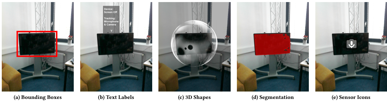
Figure 3: PriView in a mobile application: We implemented five types of visualisation, namely a) Bounding Boxes (framing the device), b) Text Labels (indicating the device’s state), c) 3D Shapes (around the device), d) Segmentation (thermal highlighting), and e) Sensor Icons (camera or microphone).
