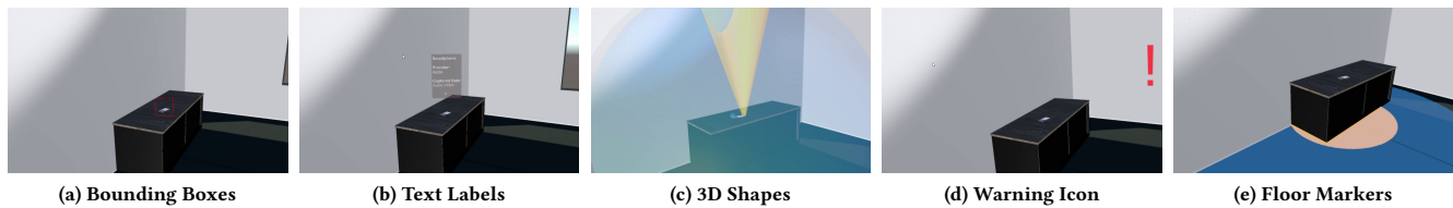
Figure 4: PriView in VR: We implemented five types of visualisation, namely a) Bounding Boxes (framing the device), b) Text Labels (indicating manufacturer, sensor and data being collected), c) 3D Shapes (highlighting the tracking space for audio: blue bubble, and video: yellow cone), d) a Warning Icon (warning), and d) Floor Markers (highlighting the tracking space for audio: blue circle, and video: yellow circle).
