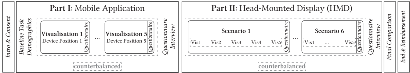
Figure 5: Study Procedure: We investigated two output devices of PriView , namely a mobile application (Part I) and a head-mounted display (Part II). We used a within-subjects design in which every participant encountered Part I and II in this order. In both parts, we explored various visualisations. For the mobile application, participants conducted a total of 6 search tasks: one without using the application (baseline) and, in counterbalanced order, one for every visualisation. Each task was followed by a questionnaire. For the HMD, participants experienced various application scenarios in counterbalanced order. Within every scenario, we counterbalanced all five visualisations. Each scenario was followed by a questionnaire. We complemented the session with an interview and a final comparison of both output devices.
