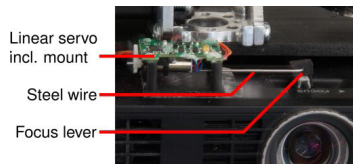
Figure 4: Implementation of the UbiBeam
