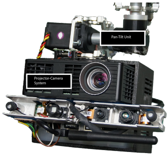
Figure 1: The UbiBeam System a Compact and Steerable Projector-Camera System
