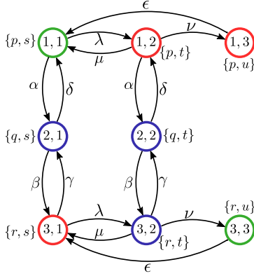
Fig. 3: Flat model with partitioned states
