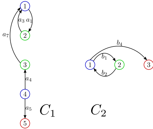
Fig. 9: Partitioned state sets in C_1 and C_2
