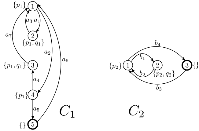
Fig. 7: Components C_1 and C_2
