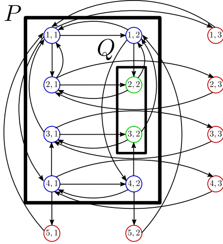
Fig. 8: Flat combined model of C_1 and C_2
