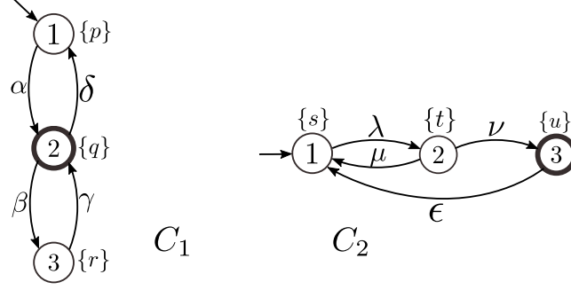
Fig. 1: CTMCs C_1 and C_2 with one resource
