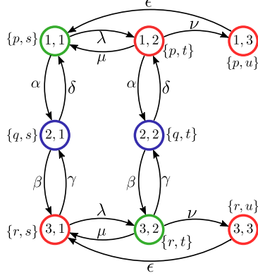
Fig. 5: Flat model with partitioned state space
