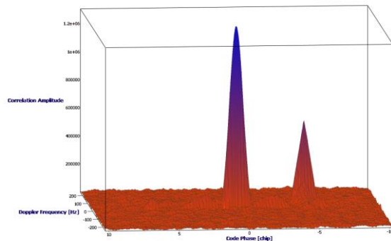
Figure 23: Multicorrelator-Plot of GPS PRN 6 when both peaks are separated by 5 chips from each other.
