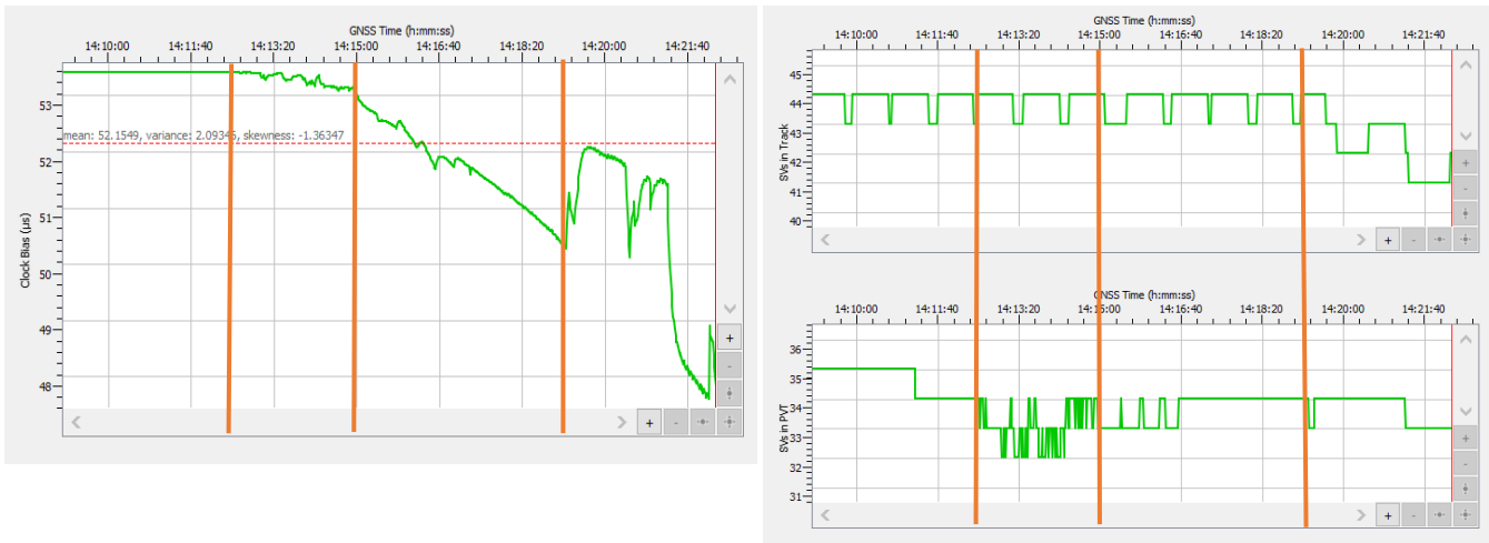
Figure 7: Septentrio PolaRx5TR, on the left side clock bias [μs] over time, on the right side upper plot satellites in tracking over time, lower plot number of satellites used for PVT over time
