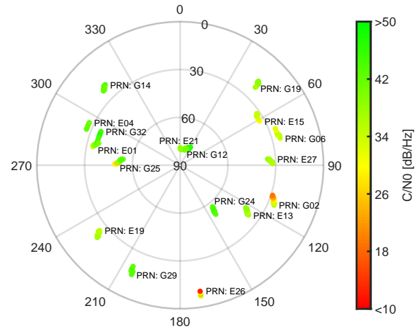
Fig. 24: Skyplot of the satellite visibility with the appropriate C/N0
