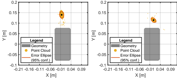
Fig. 28: Approximated APC from RTK-fixed solution from device n^{\circ}2 using two different data sets. day 1 (left) and day 2 (right)
