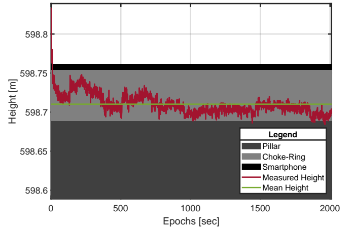
Fig. 30: Approximated APC height component from RTK-fixed solution for device n^{\circ}1 , day 1
