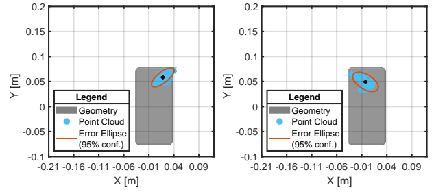
Fig. 29: Approximated APC from RTK-fixed solution from device n^{\circ}3 using two different data sets. day 1 (left) and day 2 (right)
