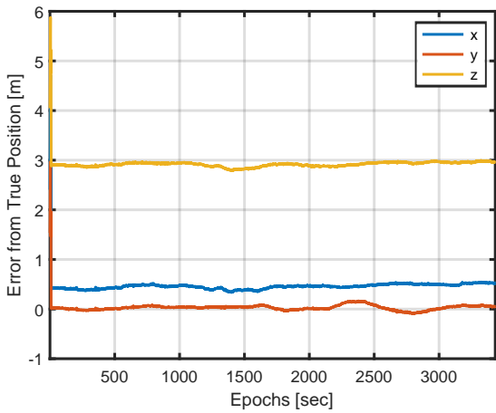
Fig. 19: RTK-Position error of Mi 8 without choke-ring
