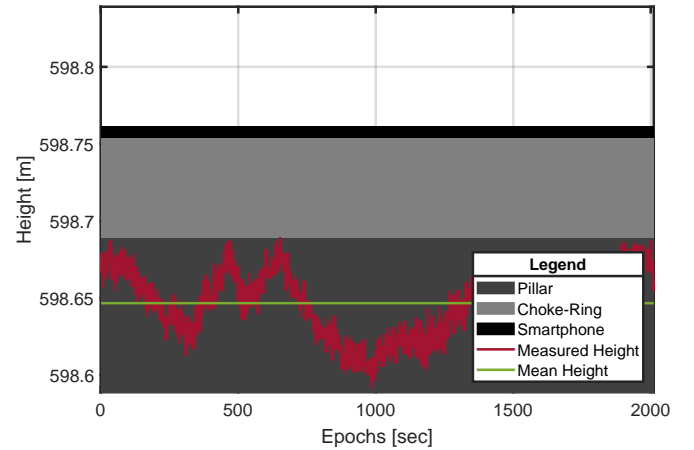
Fig. 31: Approximated APC height component from RTK-fixed solution for device n^{\circ}1 , day 2 (only float solution was possible)
