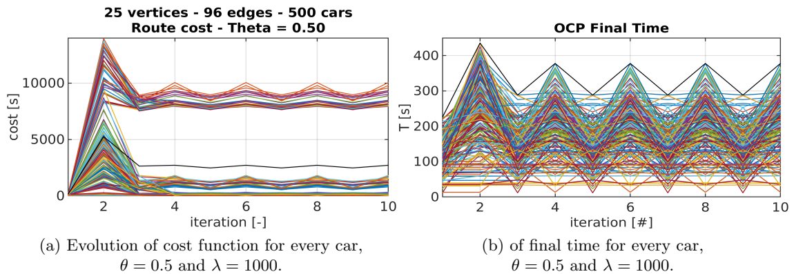
Figure 2: Numerical results for the cost function and final time over 10 iterations, n_c = 500 cars
