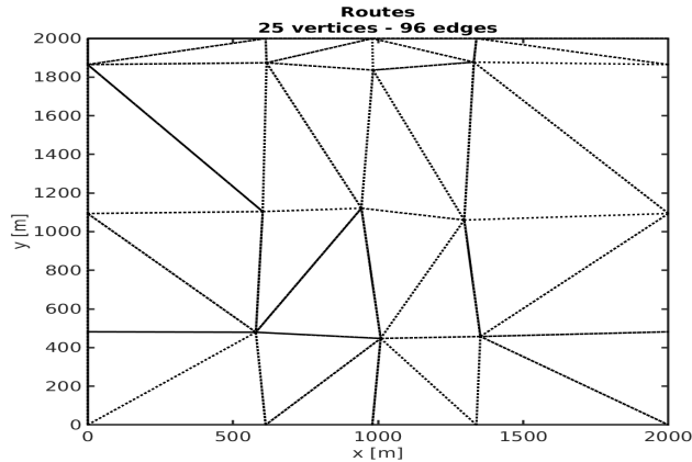
Figure 1: Randomly generated road network, connections through Delaunay triangulation.
