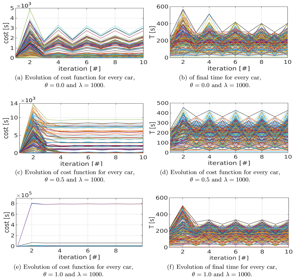
Figure 4: Implication of the hyper-parameter \theta \in [0.0; 0.5; 1.0] on the cost function and final times, with fixed \lambda = 1000 , n_c = 400 and 25 vertices - 96 edges.
