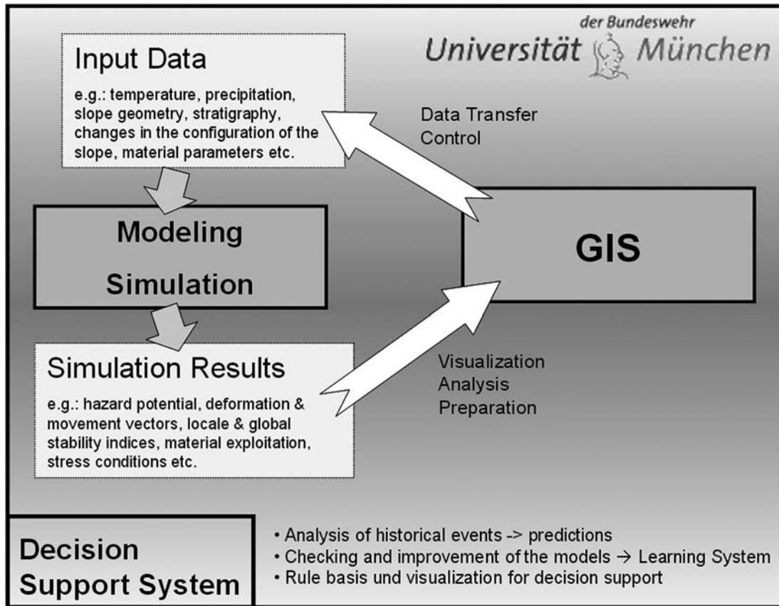
Figure 4: Interconnection between simulation system and GIS
