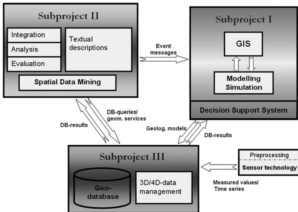
Figure 3: Overall Architecture
